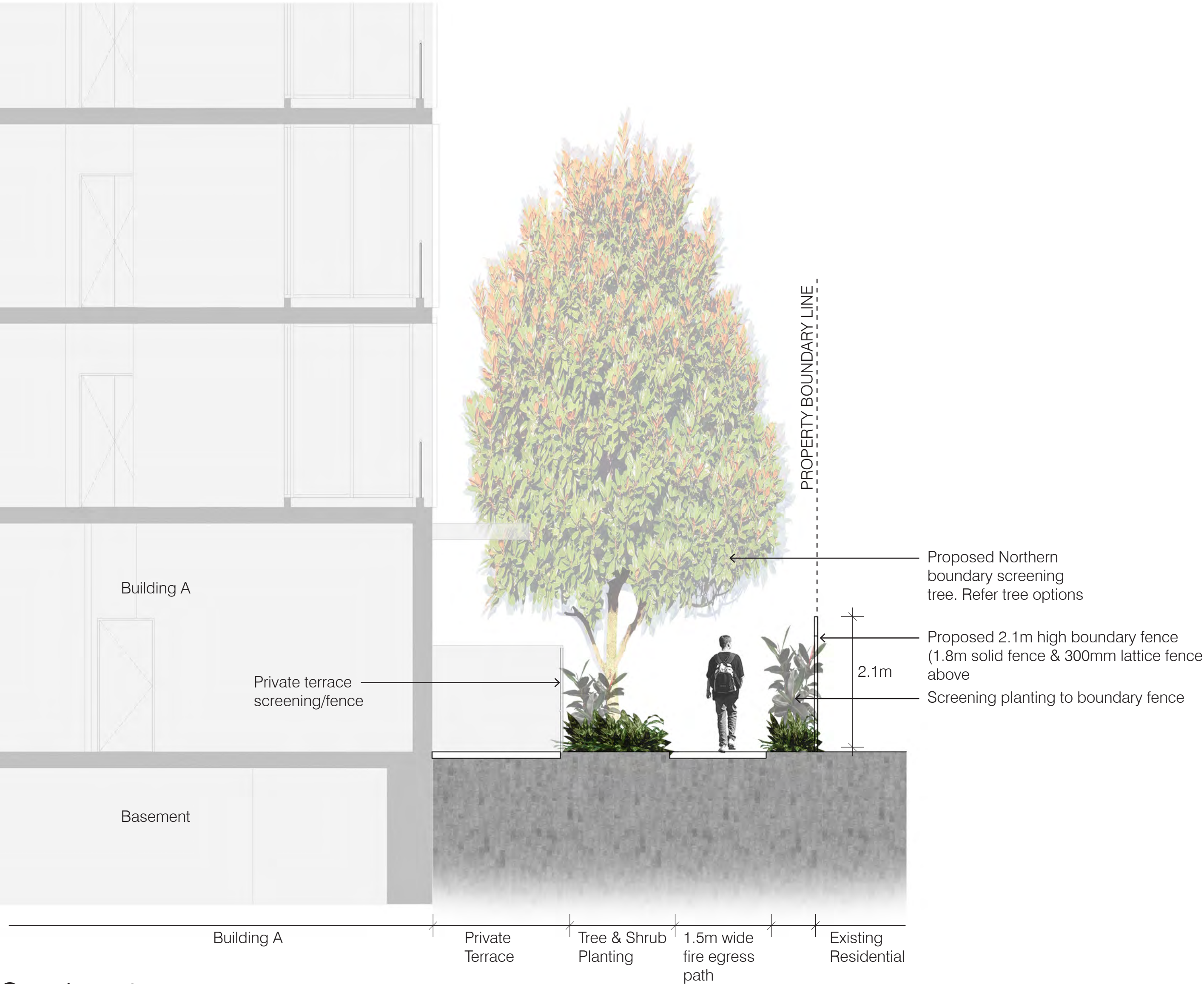
Section 1 Scale 1:50 @ A1, 1:100 @ A3
